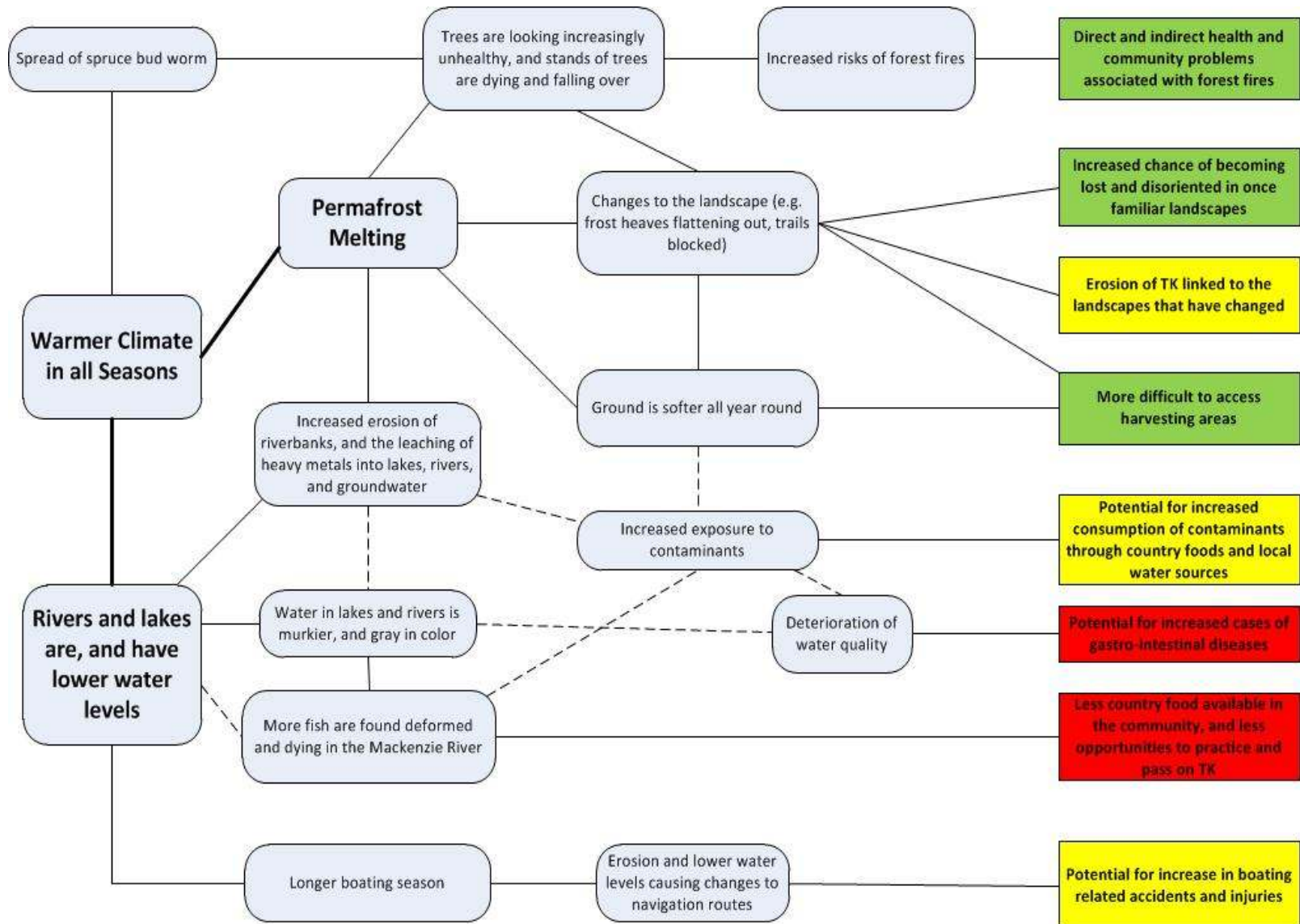
Figure 4: Influence Diagram 3 – Impacts to the Environment caused by a Warmer Climate in all Seasons
