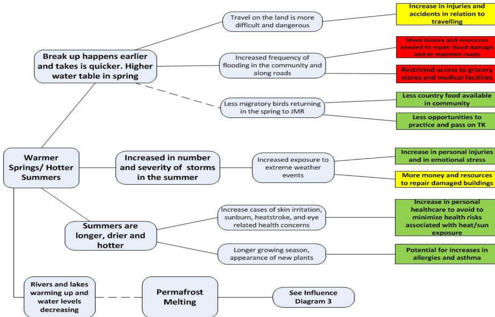
Figure 3: Influence Diagram 2 - Warmer Springs & Hotter Summers
