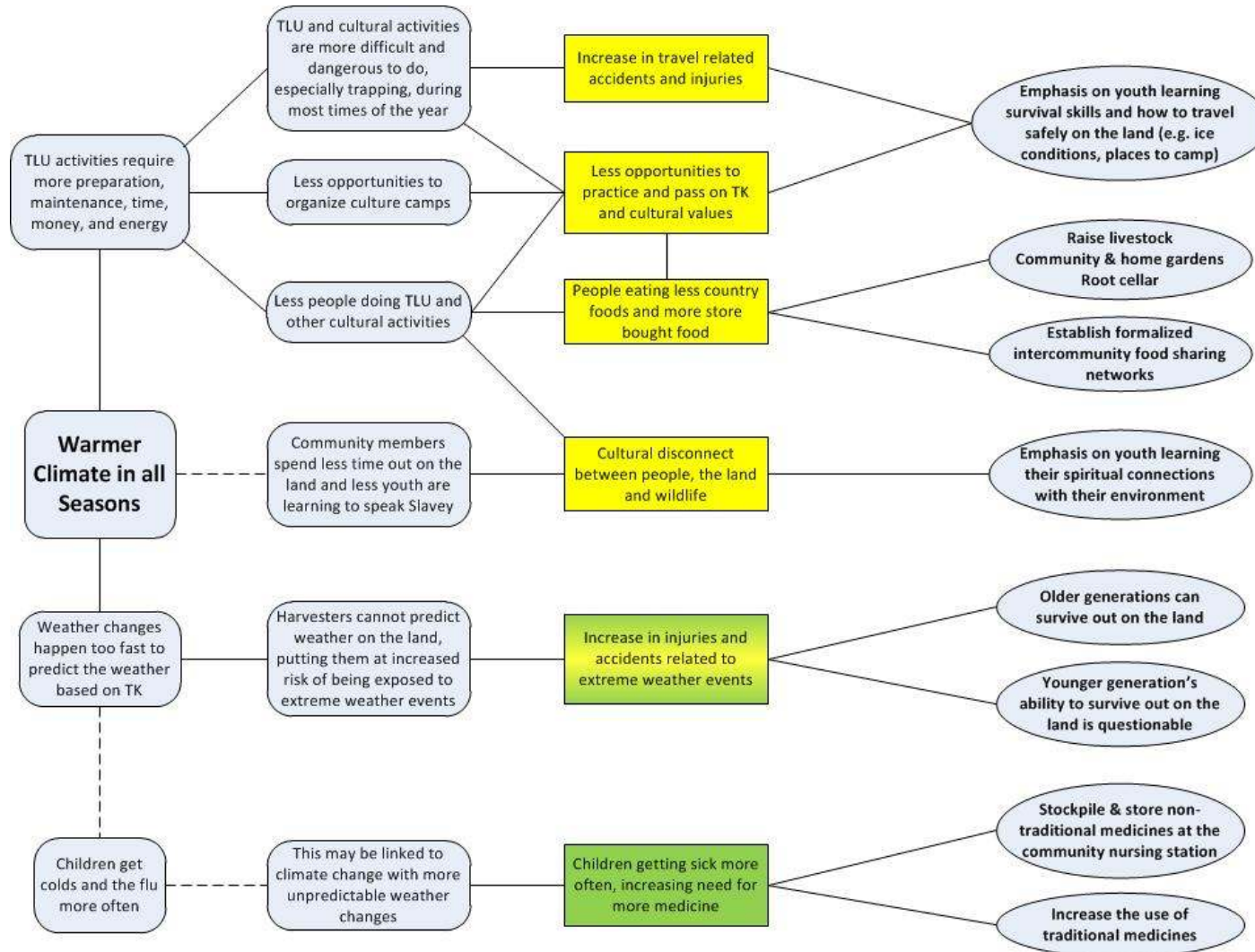
Figure 5: Influence Diagram 4 – Impacts to JMR caused by a Warmer Climate in all Seasons
