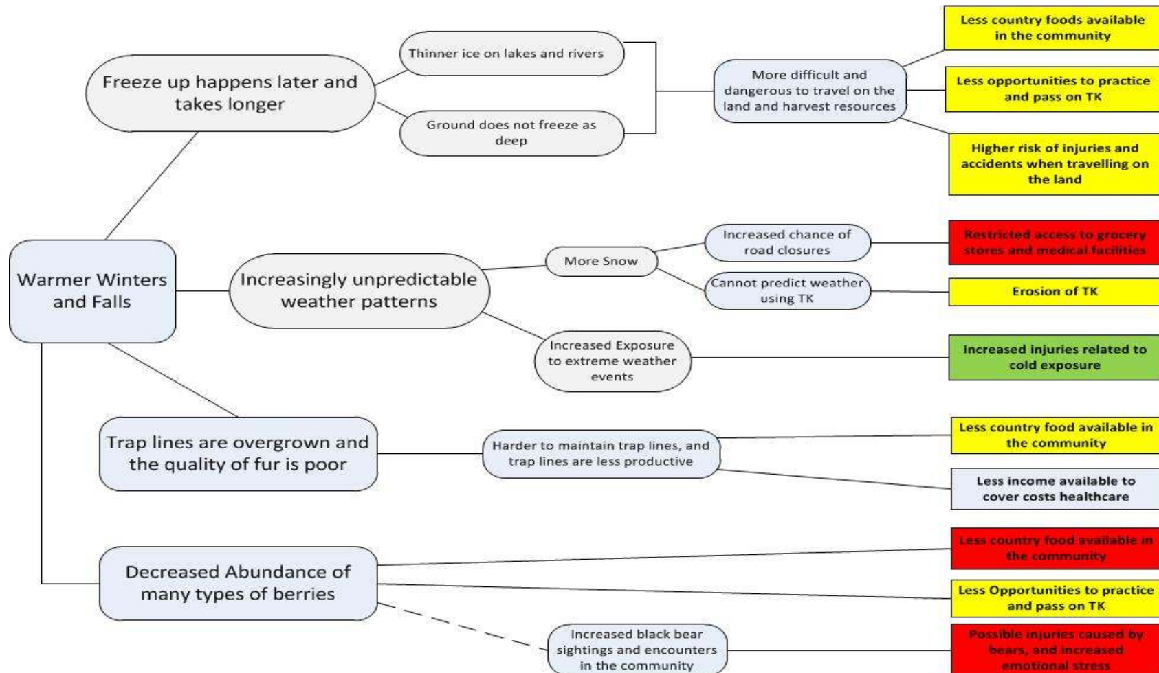
Figure 2: Influence Diagram 1 – Warmer Winters & Autumns
